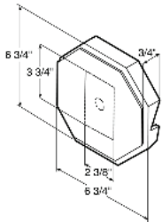
EZBLK080 Octagon Surface Mount (Double 4" or Double 5")
