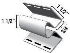
#364 Inside Corner Post
