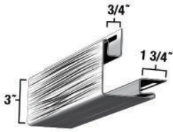
#40022 3" Outside Corner Post
