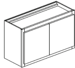
Double Door Wall Cabinet 18" High, 12" Deep
