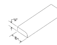
Scribe Moulding
