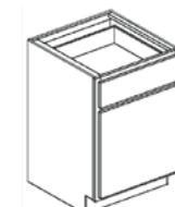
Single Door with Drawer Base Cabinet
