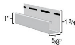
#40026 5/8" J-Channel
