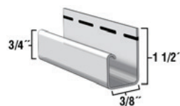
#304 3/8" J-Channel
