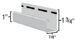
#40024 7/8" J-Channel
